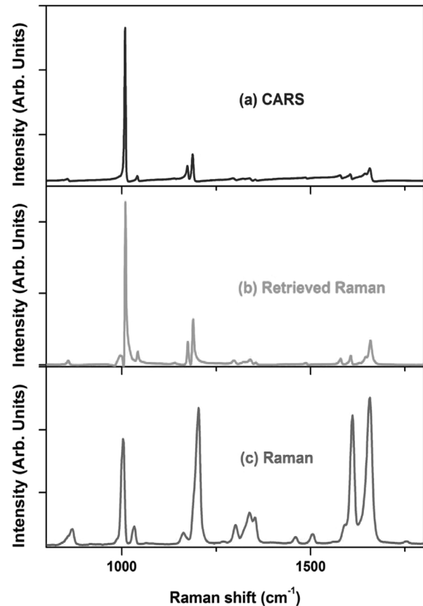
Fig. 9 (a) CARS, (b) retrieved Raman, and (c) experimentally measured Raman ( \lambda_{\text{excitation}} = 532 \text{ nm} ) spectra of a trans-stilbene solution (100 mM). Retrieval procedure was modified to take into account relatively weak non-resonant background.
