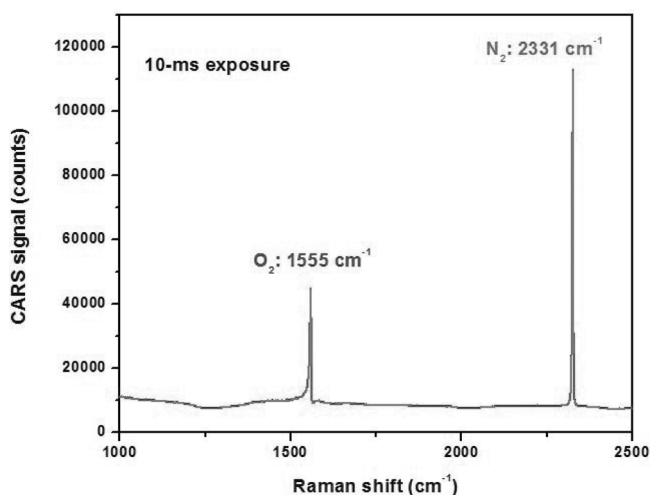
Fig. 7 CARS spectrum of the ambient air. Lines corresponding to molecular oxygen and nitrogen are clearly identified. See text for additional experimental details.
