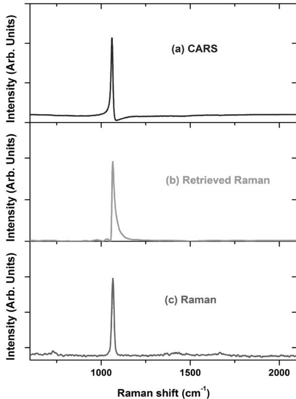
Fig. 8 (a) CARS, (b) retrieved Raman, and (c) experimentally measured Raman ( \lambda_{\text{excitation}} = 532 \text{ nm} ) spectra of a concentrated (100 mM) sodium nitrate solution. Retrieved Raman spectrum shows amended shape of the Raman line.
