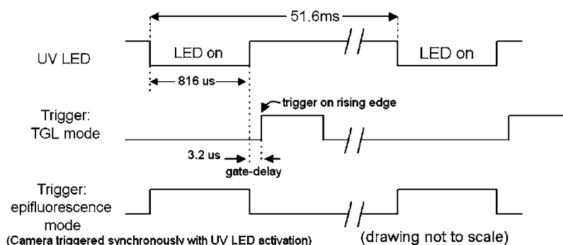
Fig. 3 Pulse timing for the UV LED and camera trigger pulse when operated in conventional epifluorescence mode (prompt). While this mode of operation uses a pulsed source, it appears continuous to the camera and eye, returning conventional fluorescence images. Rise time of the LED pulse on turn-off was 1.33 \text{ V}/\mu\text{s} ; the camera was triggered about 3.2 \mu\text{s} after the LED pulse. This small gate-delay resulted in a loss of about 1% of the initial intensity of the europium label at the moment of acquisition.
