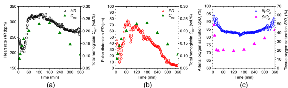
Fig. 11 Time courses of (a) HR and total hemoglobin concentration C_{\text{HbT}} ; (b) PD and total hemoglobin concentration C_{\text{HbT}} ; and (c) percutaneous arterial oxygen saturation \text{SpO}_2 and tissue oxygen saturation \text{StO}_2 for rat after the administration of \text{NaNO}_2 at a dose of 37.5 mg/kg. HR, PD, and \text{SpO}_2 were measured by the commercial existing pulse oximeter, whereas C_{\text{HbT}} and \text{StO}_2 were obtained by the proposed method.
