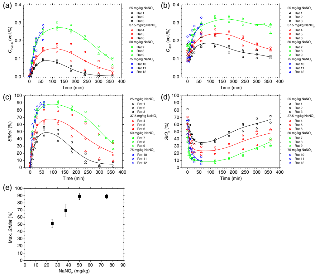
Fig. 10 Time courses of (a) methemoglobin concentration C_{\text{methHb}} ; (b) total hemoglobin concentration C_{\text{HbT}} ; (c) methemoglobin saturation StMet; and (d) tissue oxygen saturation StO 2 for various doses of NaNO 2 . (e) Relationship between the maximum value of StMet and the NaNO 2 dose. Data were obtained by the proposed method. Solid lines in (a)–(d) are means of three rats for each dose group. Plots and error bars in (e) show means and SDs of three rats for each dose group.
