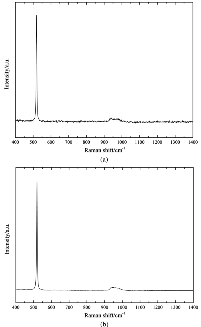
Fig. 3 Raman spectra of silicon wafer collected from (a) optical fiber excitation Raman spectrometer and (b) bench-mounted Raman spectrometer.
