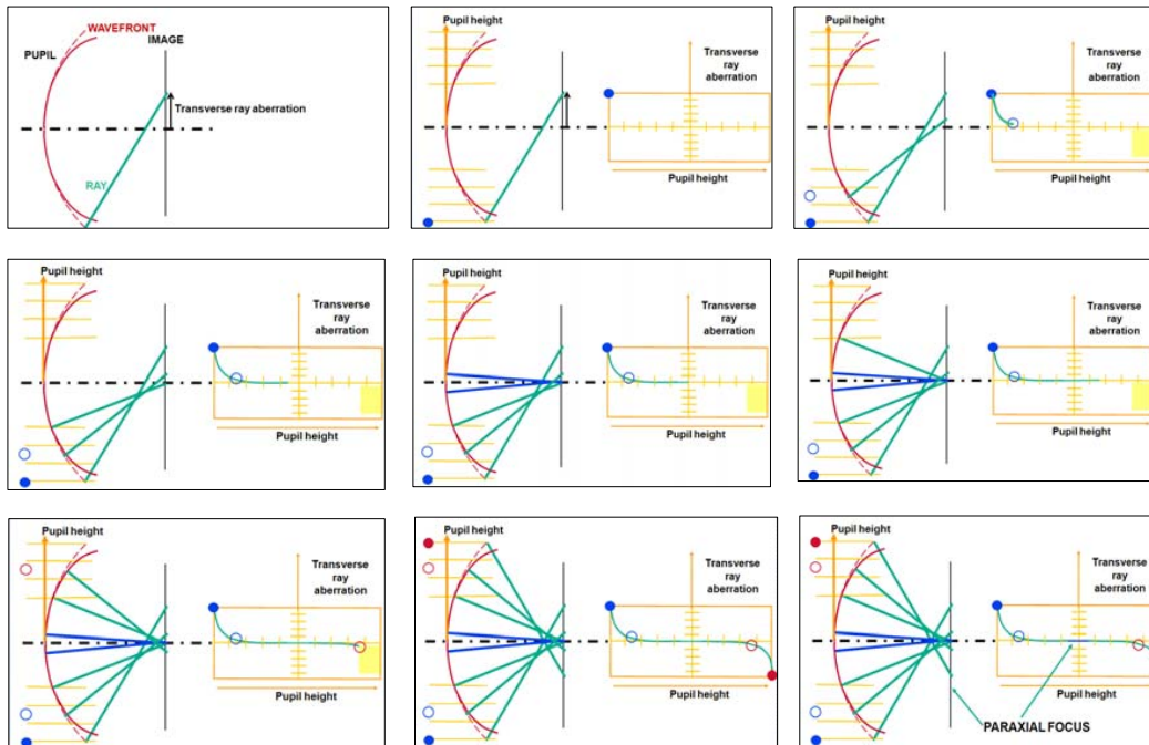
Figure 2 Sequence of slides for rapid presentation to illustrate the transverse ray aberration plotted as a function of pupil height
