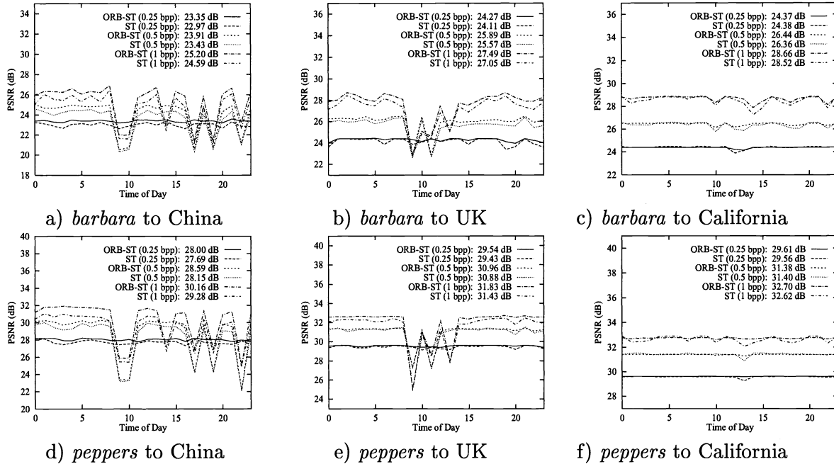
Figure 5. Comparisons of reconstruction quality for image barbara and peppers over a 24-hour period for the transmissions from Urnaba to three remote sites, when each image was coded at, respectively, 0.25 bpp, 0.5 bpp, and 1 bpp, and placed in 16, 32, and 64 packets for transmission.
