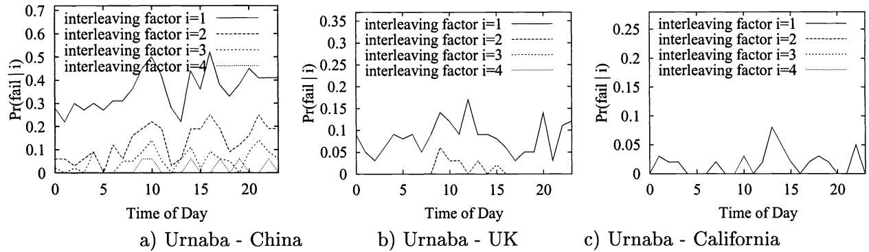
Figure 2. Pr(fail|i) , probability of bursty losses that cannot be recovered, conditioned on interleaving factor i , at different times on April 8, 2001.
