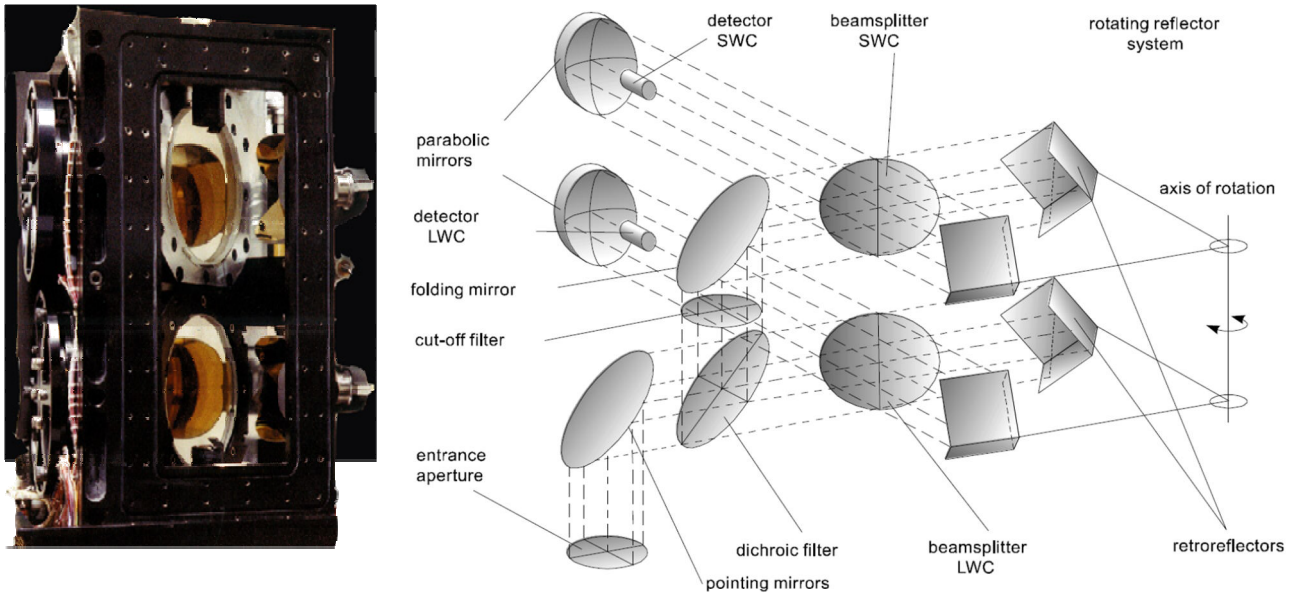
Figure 4. Left: PFS Engineering Model; Right: Optical design of PFS 56 .
