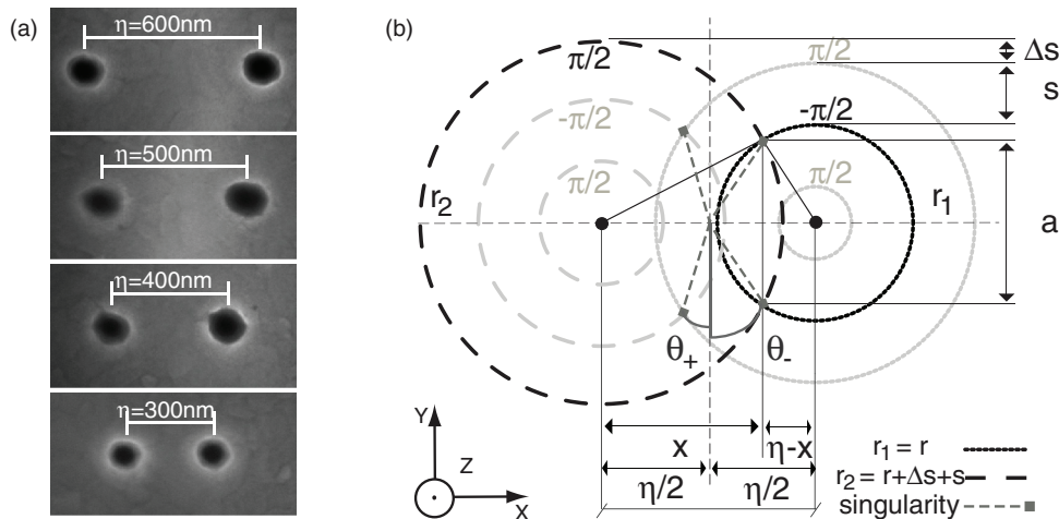
Fig. 1 In (a), SEM images of pair of nanoholes drilled by FIB in aluminum film at 100, 000 \times magnification. The images show nominal center-to-center pitches \eta of 600, 500, 400 and 300 nm with according scale bars. In (b), schematic illustration of image plane in phase with \Delta\phi \neq 0 . Circles show contours of equal phase emitted from two point sources located in the circles' centers.
