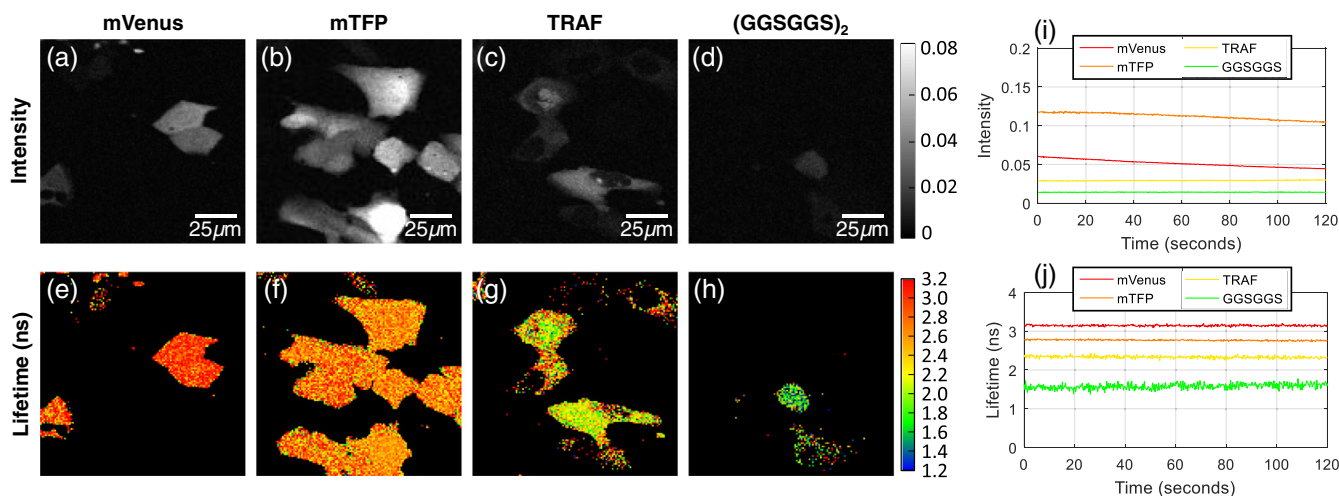
Fig. 4 High-speed imaging and photostability measurements with 25 \mu\text{W} at the sample (Nikon 0.85 NA 60\times objective). (a)–(d) Representative intensity images for cells with the fluorescent proteins and control constructs. (e)–(h) Corresponding fluorescence lifetime images. (i) Plots of intensity over time and (j) lifetime over time for a region of interest within a cell. All images are captured with 128 \times 128 points at \sim 9 fps ( 6.8\text{-}\mu\text{s} pixel dwell time). mVenus in (a) is excited with 520 nm and detected within the emission band centered at 559 nm, whereas mTFP, TRAF, and (\text{GGSGGS})_2 are excited with 450 nm and detected within the emission band centered at 479 nm.
