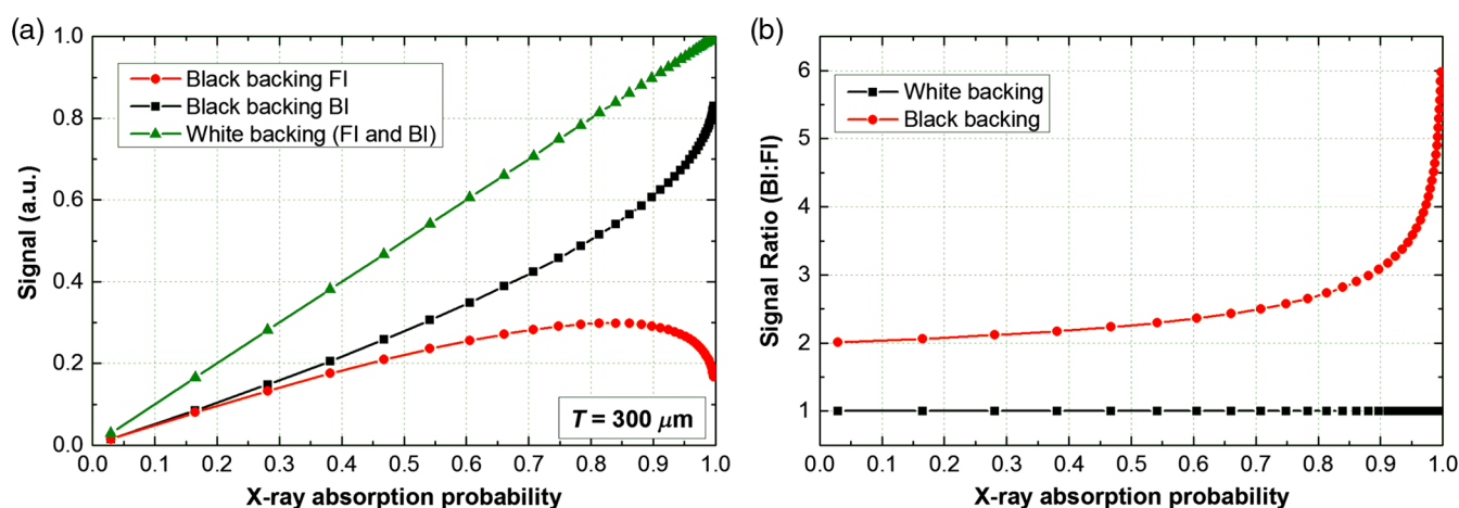
Fig. 3 Comparison of (a) DC signal for a single screen ( T = 300 \mu\text{m} ) with white or black backing, in FI and BI, for a given exposure. (b) The corresponding ratio of BI:FI signal.
